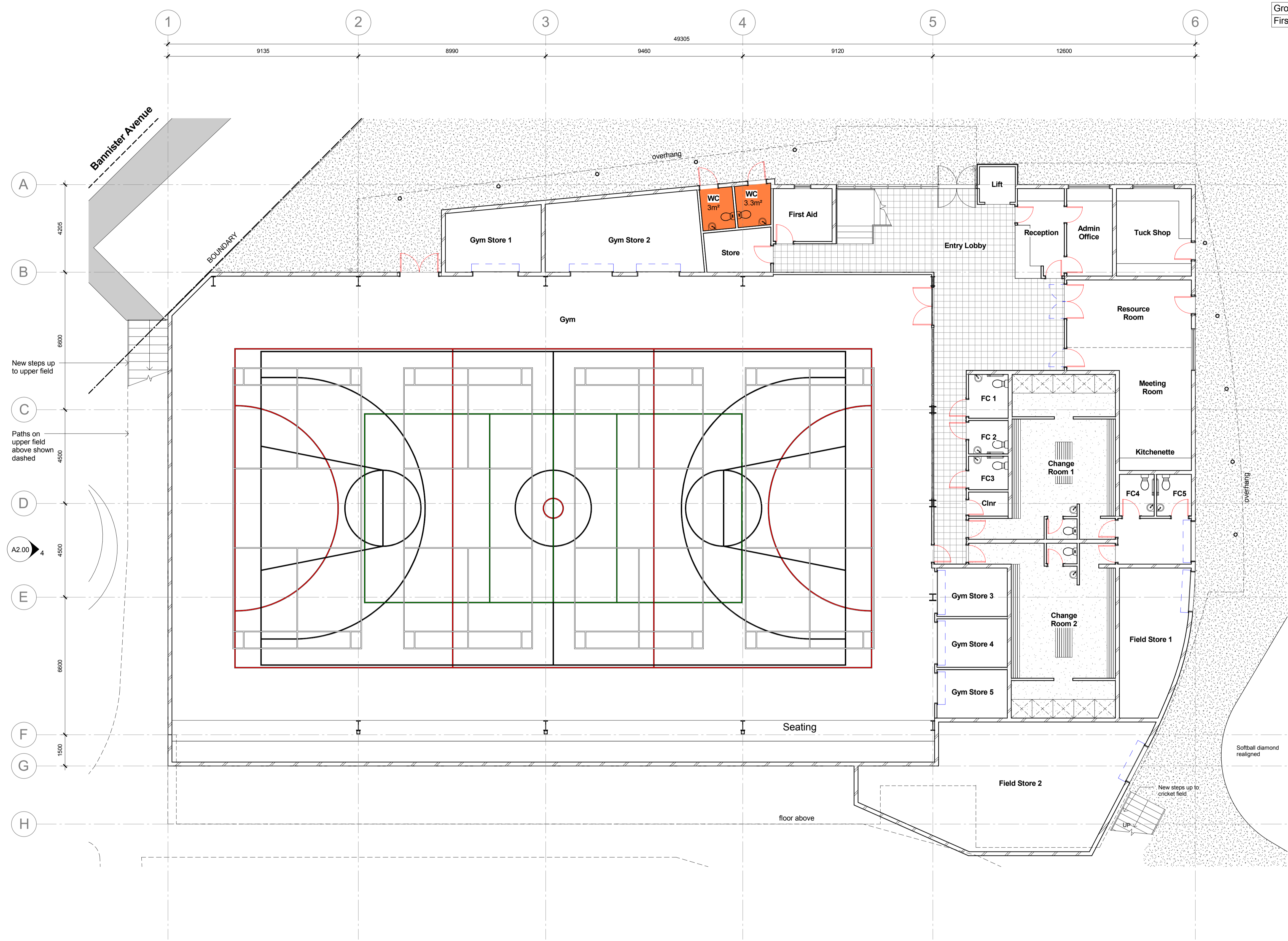
1 Proposed Ground Level A2.00 1 : 100
